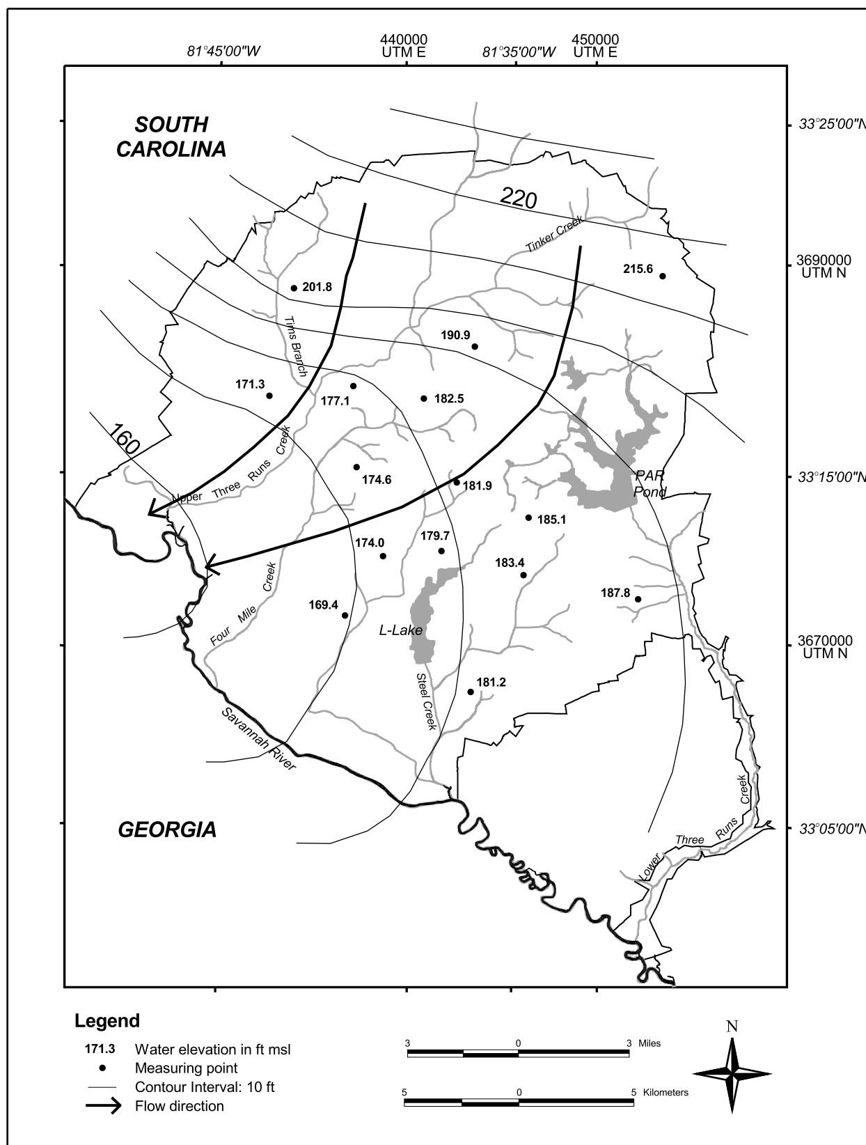
Figure 20 Potentiometric Surface of the McQueen Branch Aquifer at SRS
