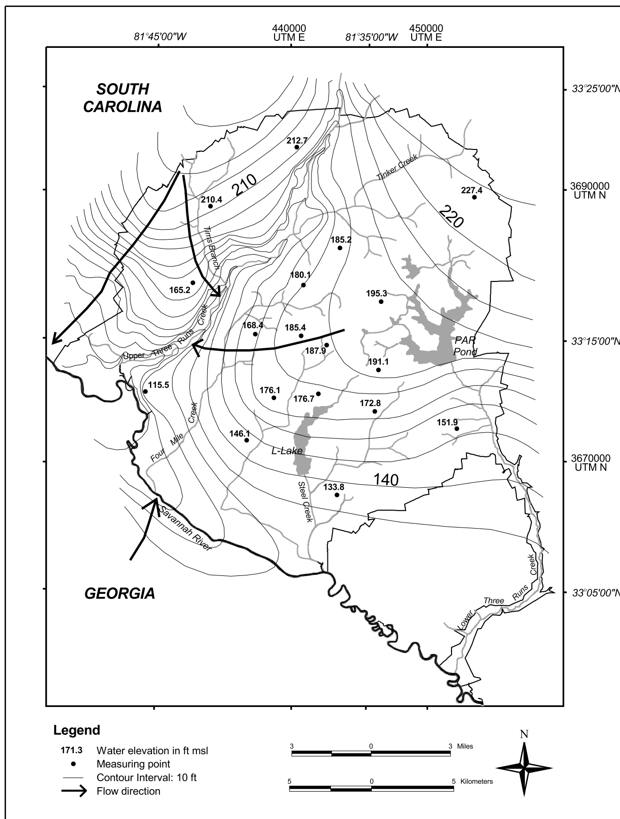
Figure 18 Potentiometric Surface of the Gordon Aquifer at SRS
