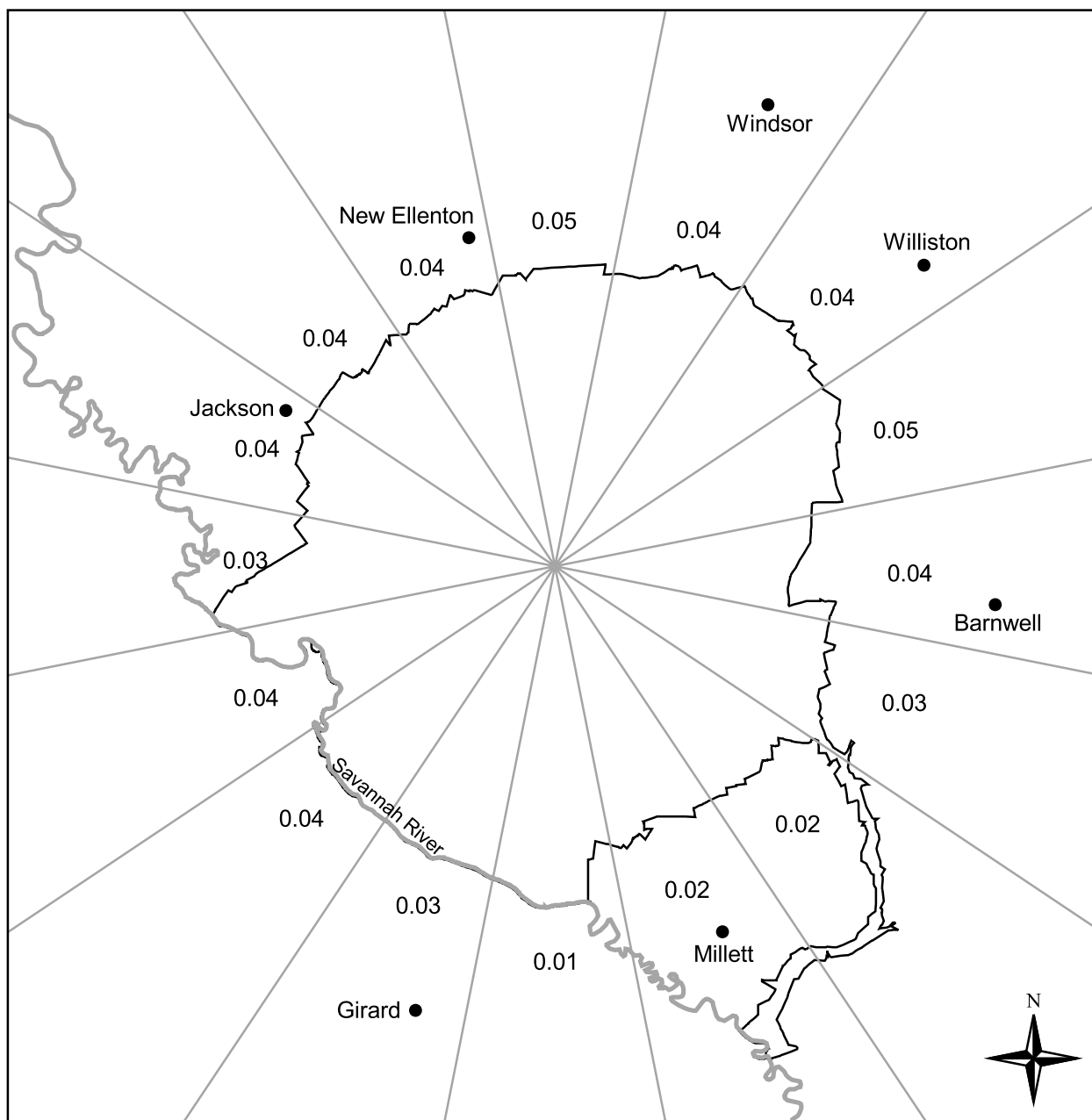
Figure 14 Sector-Specific Adult Maximally Exposed Individual Air Pathway Doses (in mrem) for 2005
