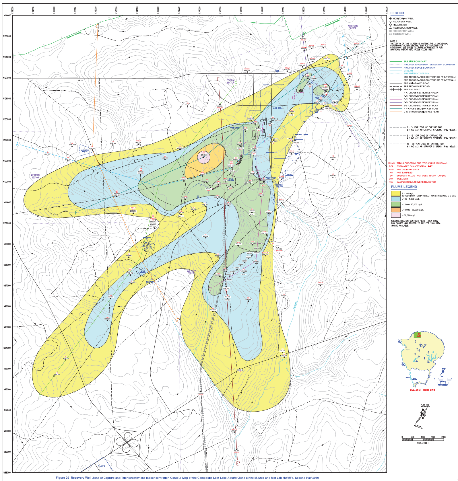
Figure 29 Recovery Well Zone of Capture and Trichloroethylene Isoconcentration Contour Map of the Composite Lost Lake Aquifer Zone at the M-Area and Met Lab HWMFs, Second Half 2010
