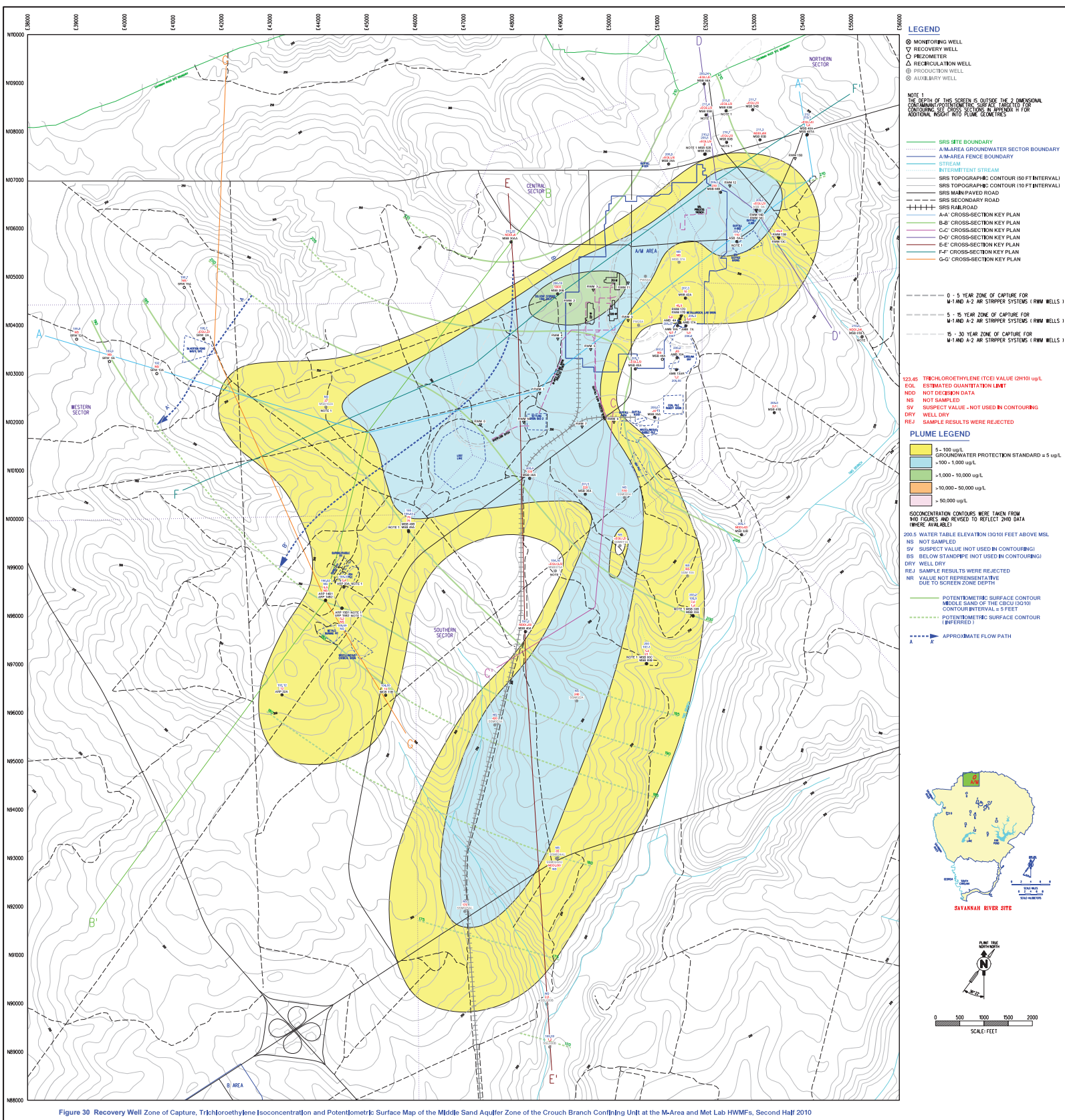
Figure 30 Recovery Well Zone of Capture, Trichloroethylene Isoconcentration and Potentiometric Surface Map of the Middle Sand Aquifer Zone of the Crouch Branch Confining Unit at the M-Area and Met Lab HWMFs, Second Half 2010
