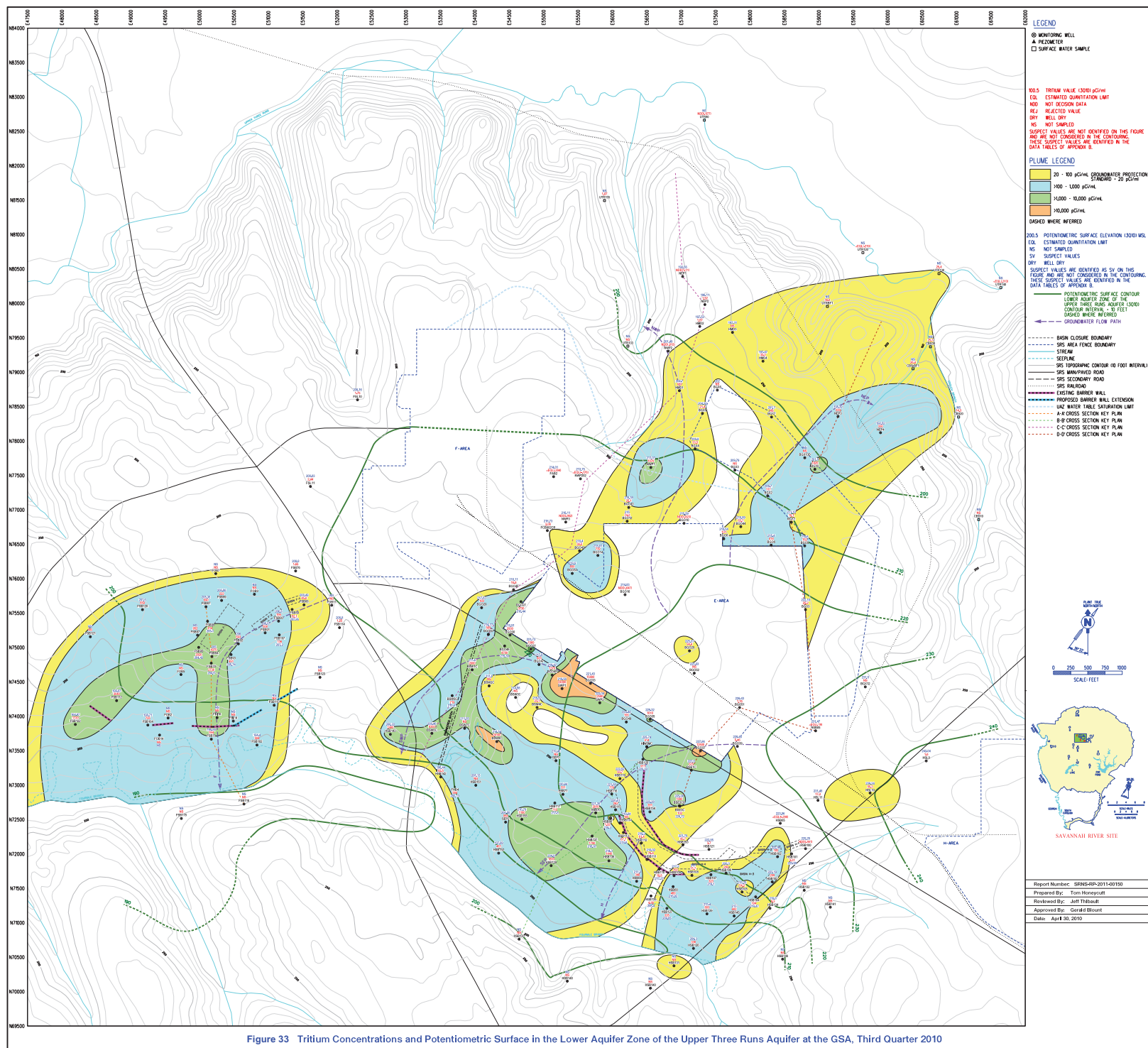
Figure 33 Tritium Concentrations and Potentiometric Surface in the Lower Aquifer Zone of the Upper Three Runs Aquifer at the GSA, Third Quarter 2010
