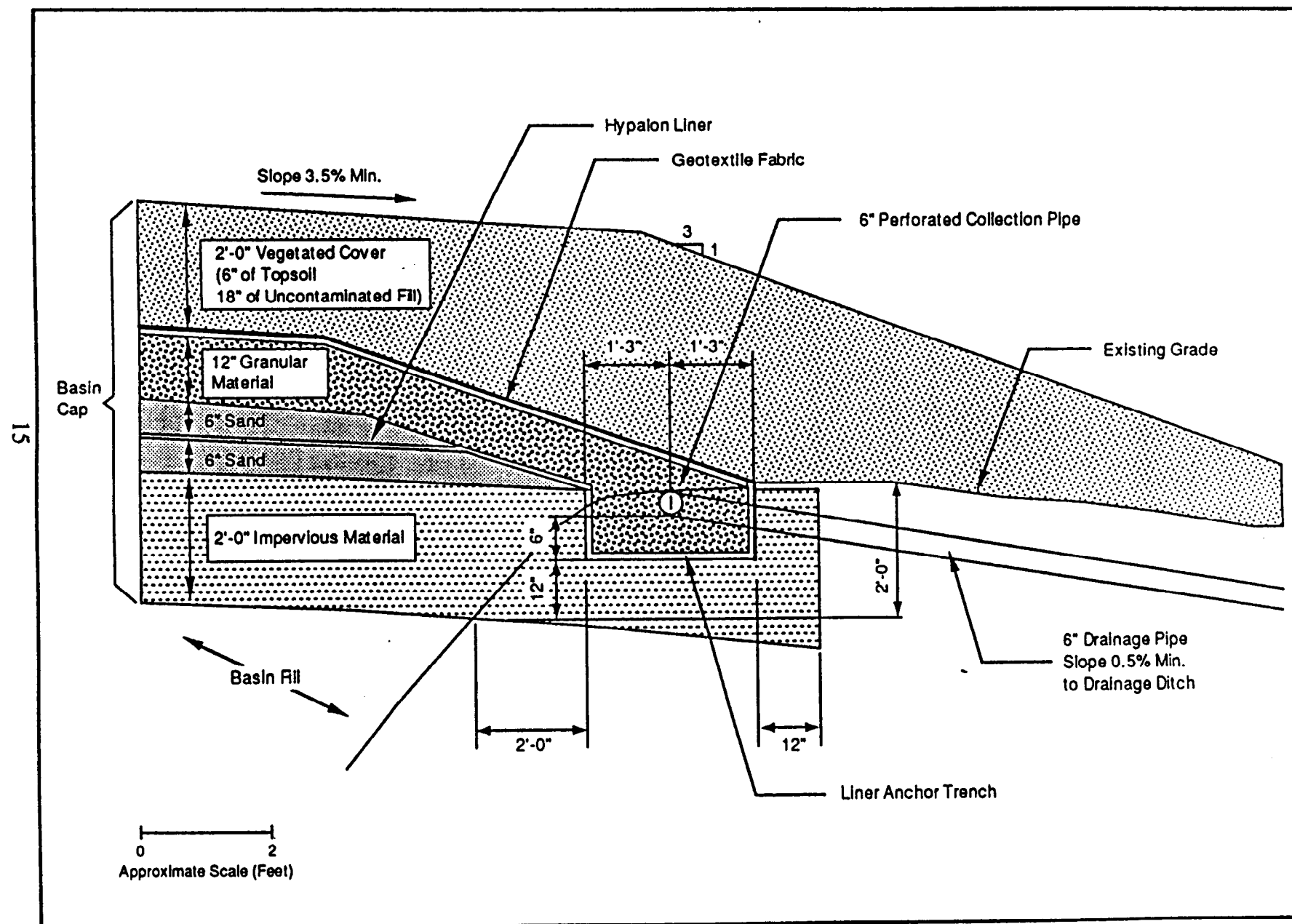
Figure 4 Schematic Diagram of the M-Area HWMF Cap
