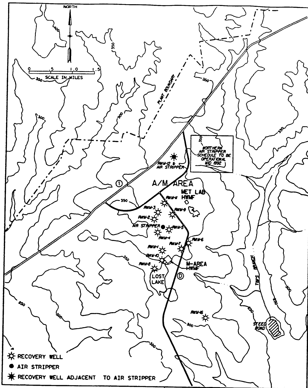
Figure 3 Location of A/M Area Groundwater Recovery Wells and Air Stripper Unit (Source: Figure created from data contained in the M-Area Hazardous Waste Management Facility Post-Closure Permit, 1991, Second Quarter Report)
