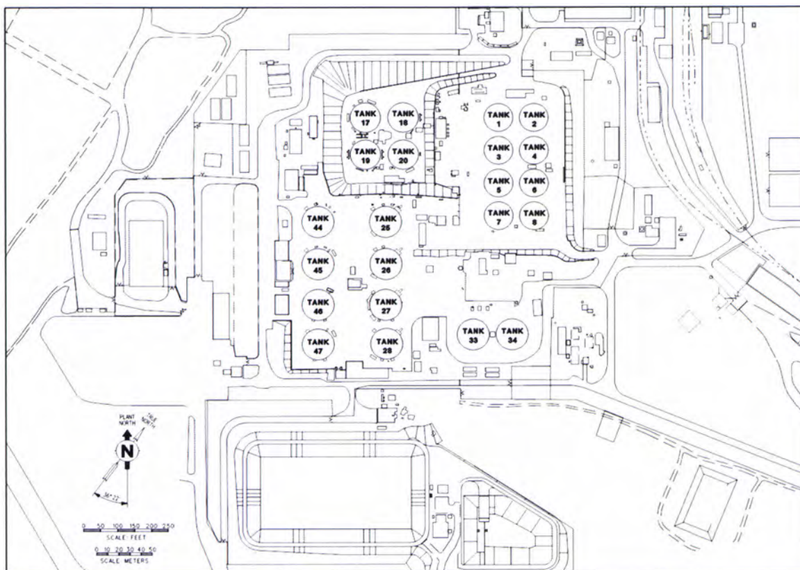
FIGURE 3: GENERAL LAYOUT OF THE F-TANK FARM
