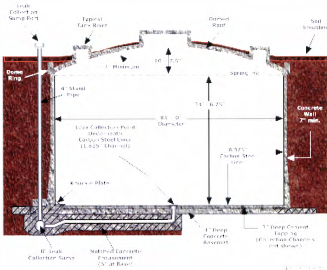
FIGURE 4: CROSS-SECTIONAL VIEW OF TYPICAL FTF TYPE IV TANK
