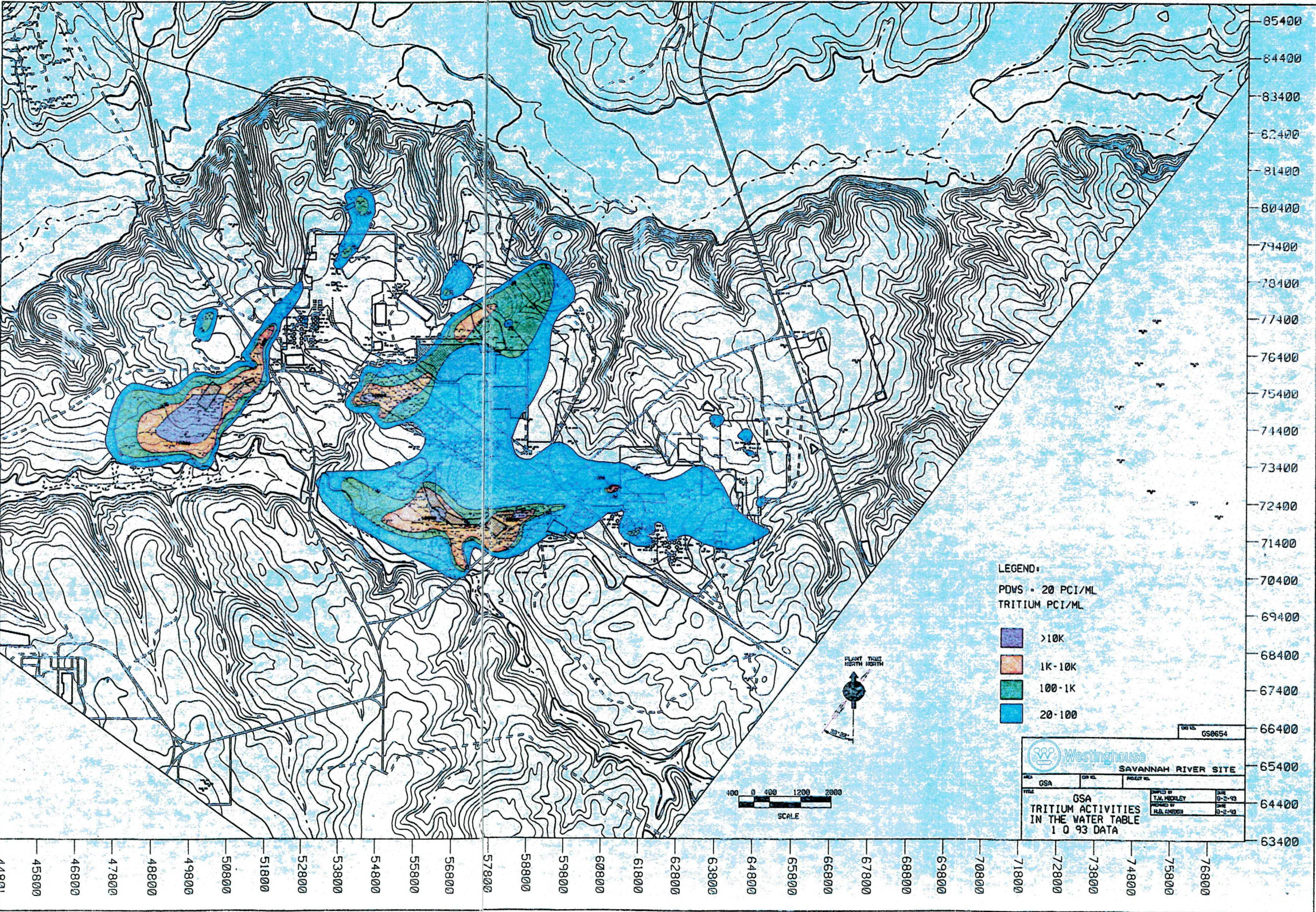
Fig. 3. Contaminant Plumes in Water Table Aquifer, F- and H-Area Groundwater Operable Units
